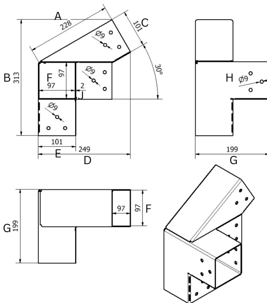
Matmenys/Dimensions, mm
